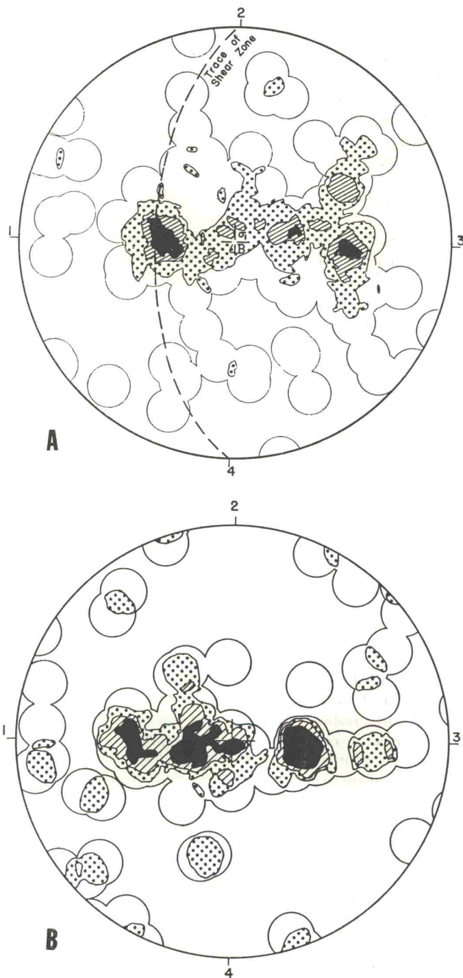
FIG. 15.— A , specimen 725. Composite diagram of normals to 102 \epsilon twin lamellae. The plane of the diagram is perpendicular to long axis of deformed cylinder, and \sigma_1 is at the center. Contours: 1, 3, 5, and 7 per cent per 1 per cent area. B , specimen 780. Composite diagram of normals to 61 \epsilon twin lamellae. The plane of the diagram is perpendicular to long axis of deformed cylinder, and \sigma_1 is at the center. Contours: 1.66, 3.33, 5.0, and 6.66 per cent per 1 per cent area.
